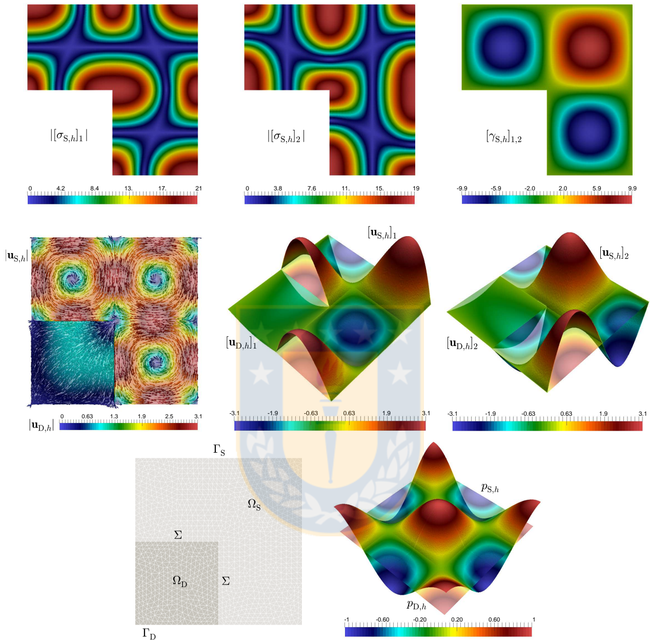
Figure 8.2: Example 2. Approximated spectral norm of the pseudostress tensor components and the skew-symmetric part of the Navier–Stokes velocity gradient (top panel), velocity streamlines and velocity components on the whole domain (middle panel), and geometry configuration and pressure field in the whole domain (bottom panel).
