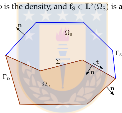
Figure 2.1: Sketch of a 2D geometry of our Navier–Stokes/Darcy–Forchheimer model
