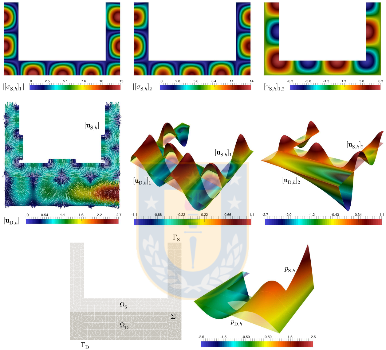
Figure 8.3: Example 3. Approximated spectral norm of the pseudostress tensor components and the skew-symmetric part of the Navier–Stokes velocity gradient (top panel), velocity streamlines and velocity components on the whole domain (middle panel), and geometry configuration and pressure field in the whole domain (bottom panel).
